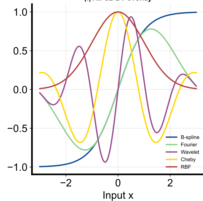
(f) All C2-BV overlay
