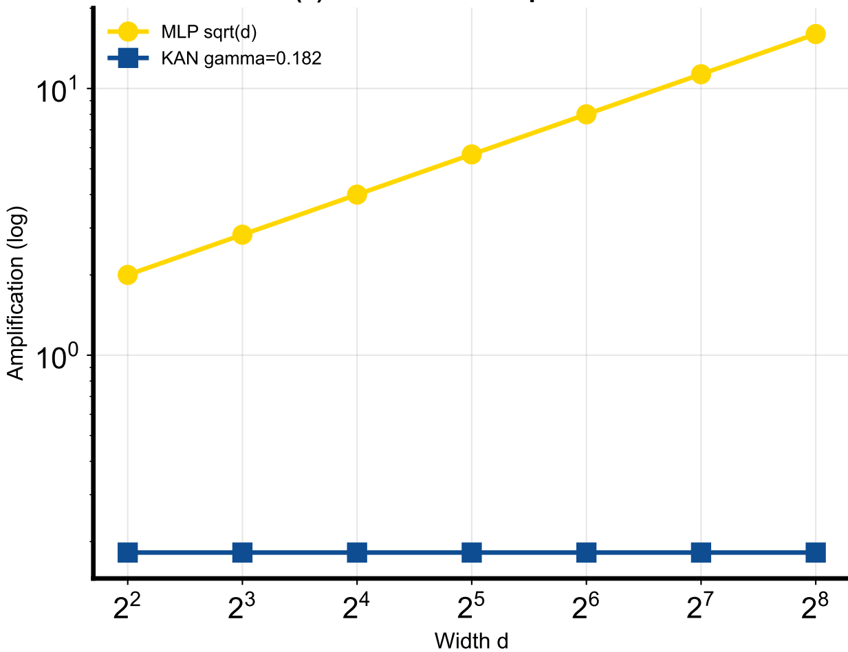
(a) MLP vs KAN amplification
