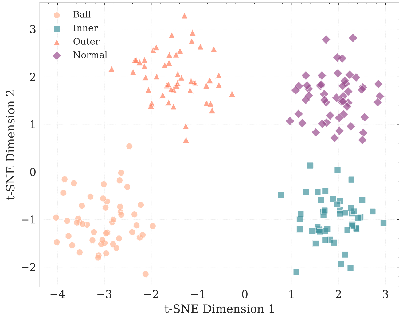
(B) VRM-KD (99.93%)
