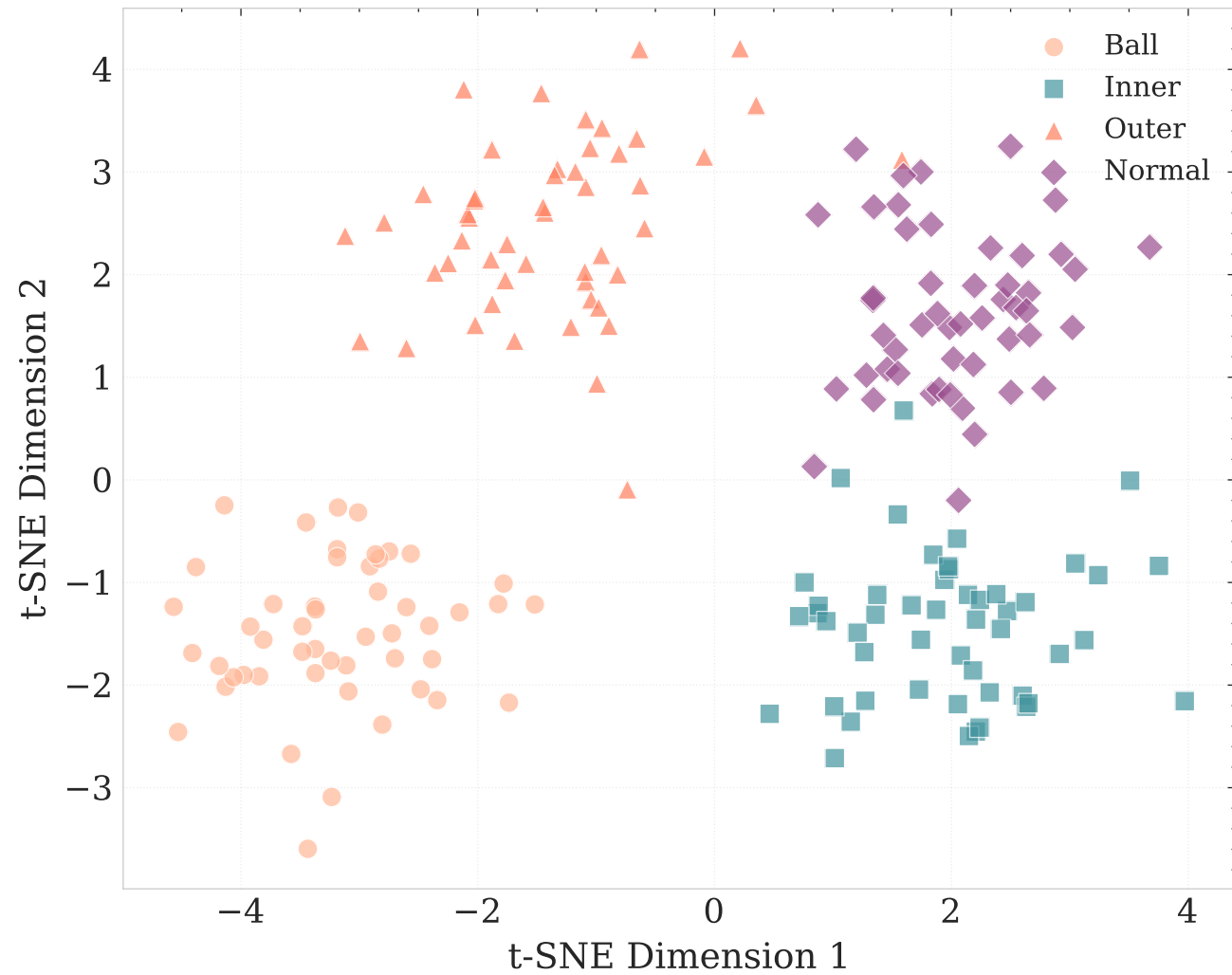
(A) No-KD (24.13%)
