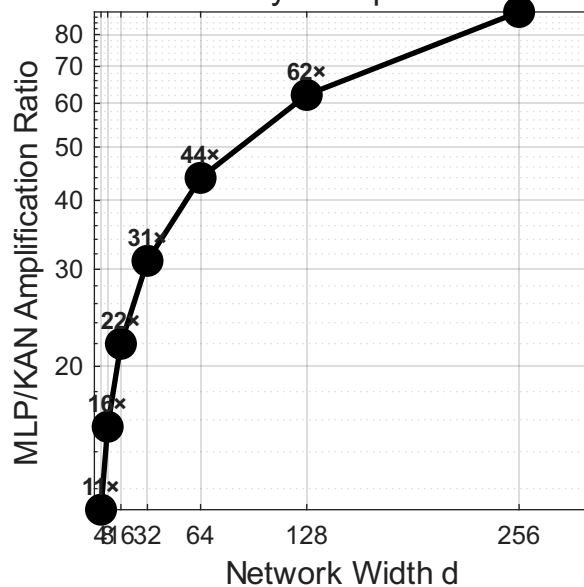
Per-Layer Gap: \sqrt{d} / 88 \times
