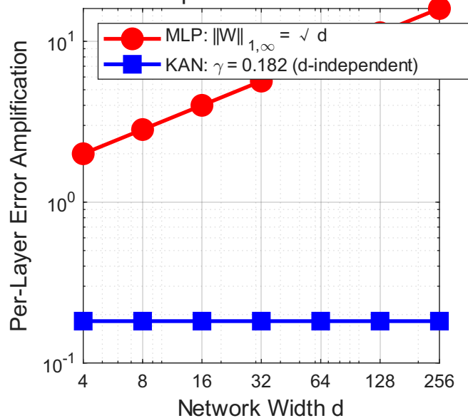
Error Amplification: MLP vs KAN
