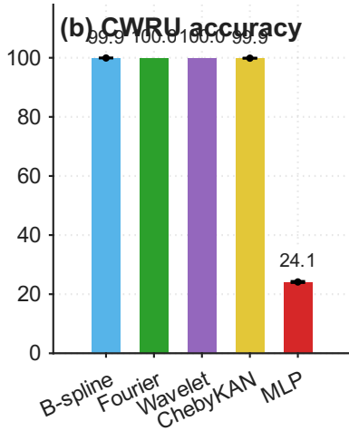
Test accuracy (%)
