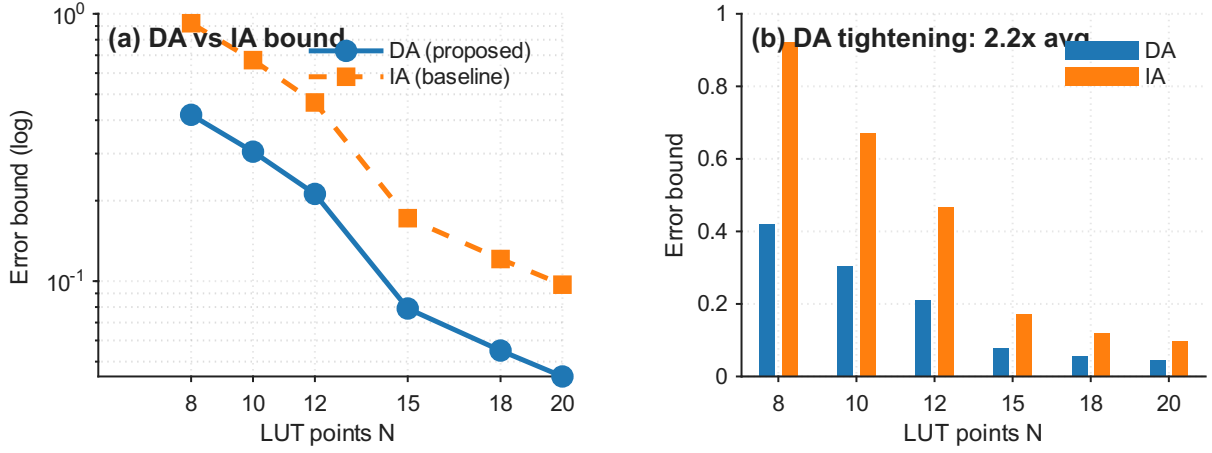
Fig. 9. DA vs. IA Bound Comparison with LUT Resolution. Left: DA achieves 2.2\times tighter bounds than IA across all LUT resolutions ( N = 8-20 ), decreasing \propto 1/N^2 (Theorem C). At N=15 : DA = 0.079, IA = 0.172. Right: bar comparison. The gap follows from DA's Galois-optimality (Theorem B).
