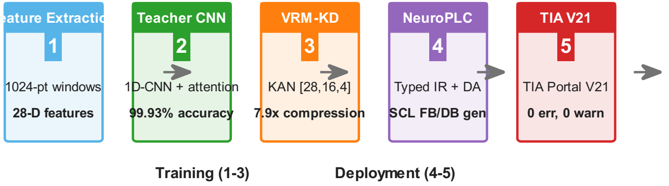
Fig. 5. NeuroPLC end-to-end pipeline. (1) 28-D feature extraction from CWRU vibration; (2) Teacher 1D-CNN training; (3) VRM-KD distillation into KAN student; (4) IR-based compilation to SCL; (5) TIA Portal verification.
