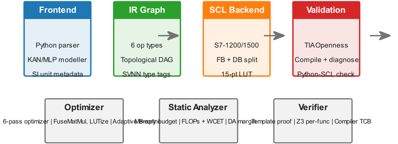
Fig. 6. Compiler architecture. Four-stage IR-based pipeline: Frontend (PyTorch \rightarrow IR) \rightarrow IR Graph (6 operation types) \rightarrow Optimizer (adaptive B-spline LUT) \rightarrow Backend (SCL code generation for S7-1200/S7-1500).
