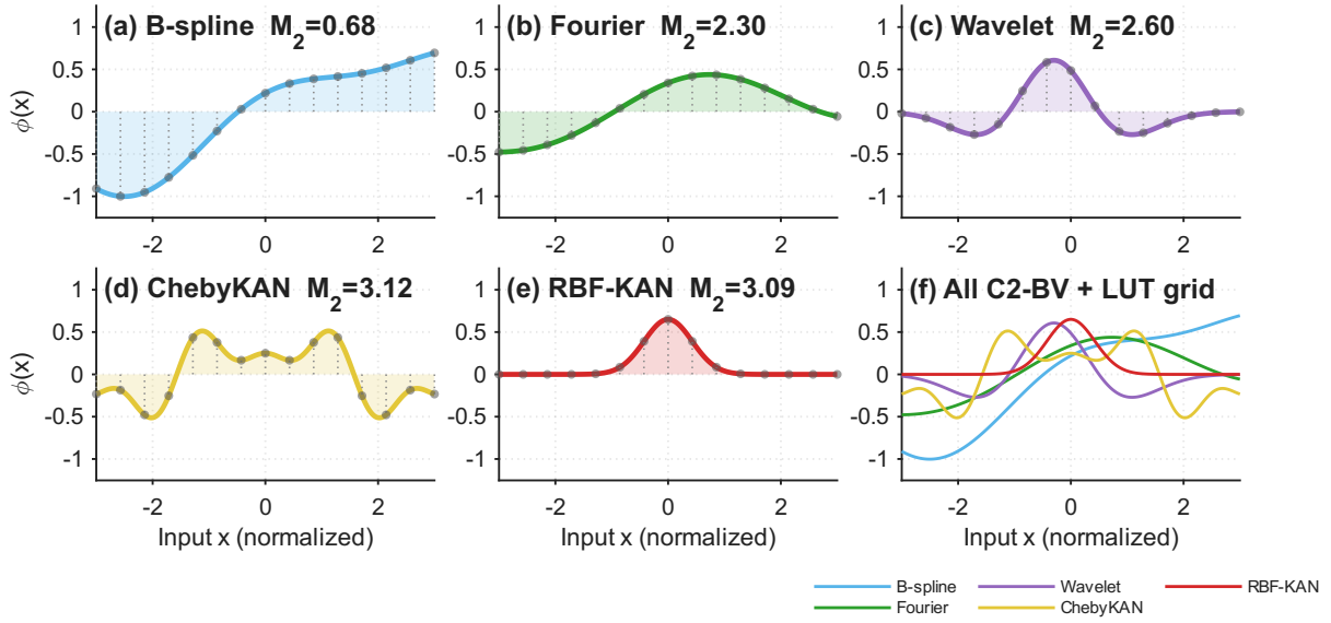
Fig. 1. C^2 -BV Architecture Family: Activation Basis Functions. Five SVNN-compliant activation function families on [-3, 3] with N=15 LUT grid points. All are C^2 with computable M_2 bounds (annotated per subplot). Despite diverse functional forms, all share the SVNN-critical property: each \phi_{j,i}(x_i) is a univariate C^2 function on a compact domain, enabling uniform LUT compilation with de Boor error bound M_2 h^2/8 (Theorem C).
