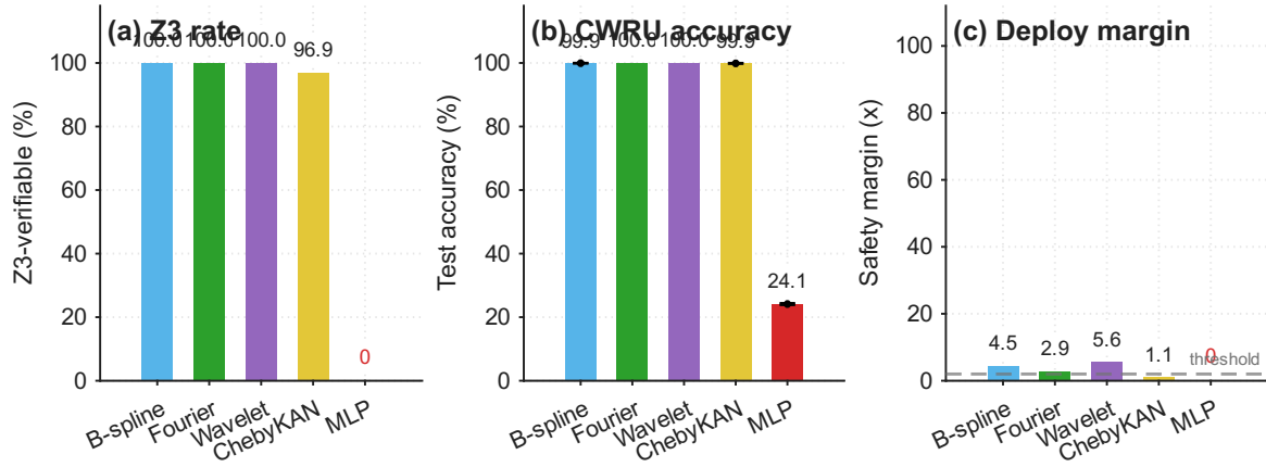
Fig. 2. C^2 -BV Architecture Family: SVNN Verification Across 5 Architectures. Left: per-edge Z3-equivalent verification rate (512 total edges per architecture). All four C^2 -BV architectures (B-spline, Fourier, Wavelet, ChebyKAN) achieve \geq 96.9\% Z3 verification; standard MLP achieves 0/48 (E41). Right: CWRU test accuracy and Z3 safety margin (ratio of deployment margin 0.182 to \max M_2 \cdot h^2/8 ). WaveletKAN's 5.6\times margin reflects M2-regularized training ( \lambda = 0.01 ). FourierKAN's M_2 is bounded by \omega^2 \sum k^2(|c_k| + |d_k|) (Proposition 5(c)). Safety margins \geq 2\times confirm deployability for all C^2 -BV architectures.
