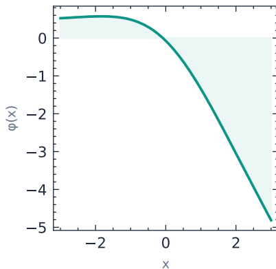
\phi[20 \rightarrow 10]
