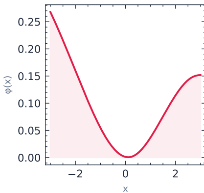
\phi[20 \rightarrow 10]
