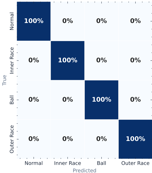
Teacher 1D-CNN (99.93%)
