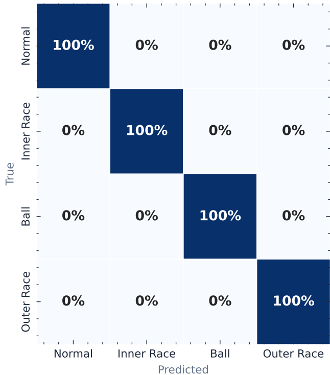
Student KAN VRM-KD (99.93%)
