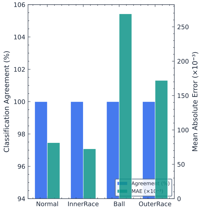
Per-Class: 100.0% Overall
