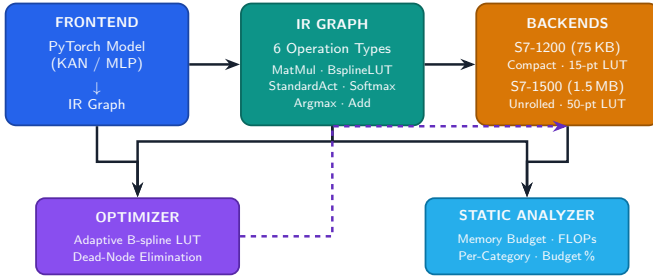
Fig. 2. Compiler architecture. Four-stage IR-based pipeline: Frontend (PyTorch \rightarrow IR) \rightarrow IR Graph (6 operation types) \rightarrow Optimizer (adaptive B-spline LUT) \rightarrow Backend (SCL code generation for S7-1200/S7-1500).
