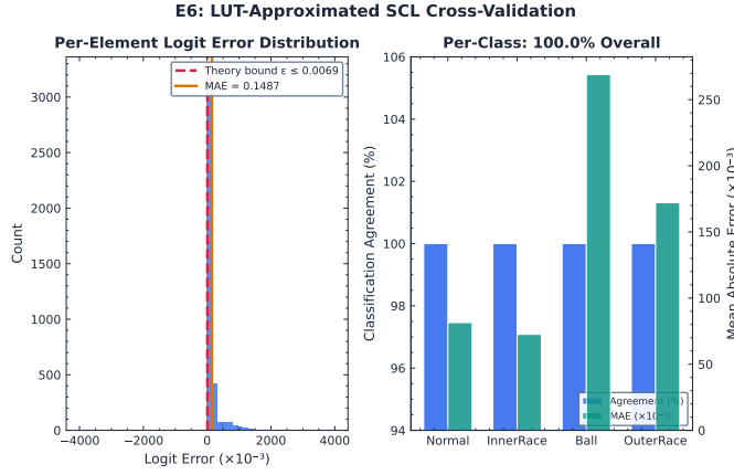
Fig. 9. E6: LUT cross-validation. Left: per-element logit error histogram (MAE 0.15, MaxAE 3.65, dominated by inter-class margins \geq 1.35 ). Right: per-class agreement (all four categories at 100%). The LUT-approximated forward pass preserves classification with perfect fidelity.
