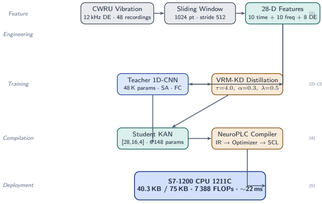
Fig. 1. NeuroPLC end-to-end pipeline. (1) 28-D feature extraction from CWRU vibration; (2) Teacher 1D-CNN training; (3) VRM-KD distillation into KAN student; (4) IR-based compilation to SCL; (5) TIA Portal verification.
