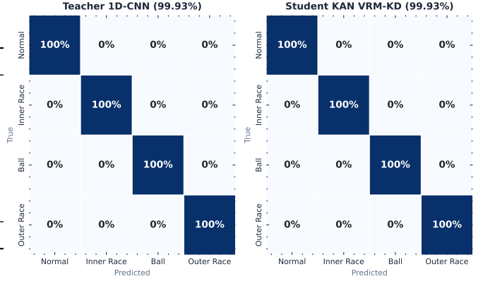
Fig. 7. Confusion matrices. Teacher 1D-CNN (left, 99.93%) and KAN student under VRM-KD (right, 99.93%) on the CWRU held-out test set (2,743 samples). Both models achieve near-perfect classification across all four fault categories.
