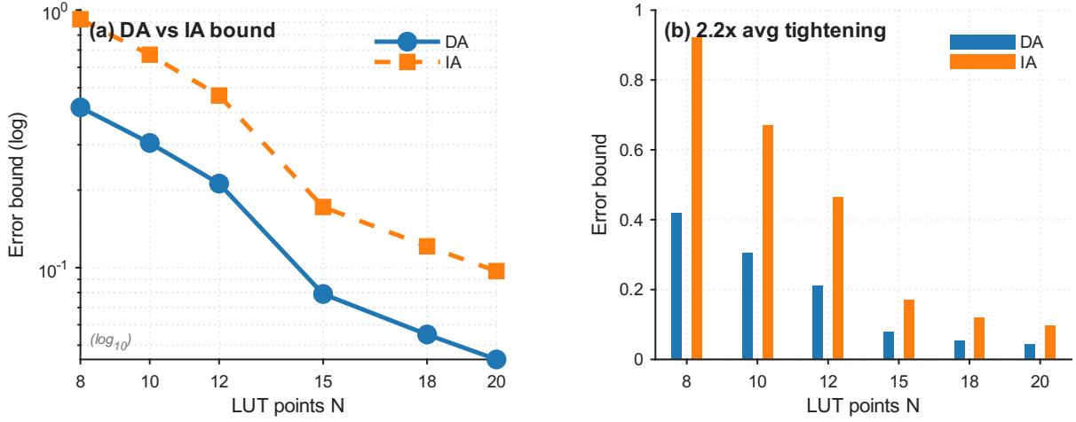
Fig. 9. DA vs. IA Bound Comparison with LUT Resolution. Left: DA achieves 2.2 \times tighter bounds than IA across all LUT resolutions ( N = 8\text{--}20 ), decreasing \propto 1/N^2 (Theorem C). At N=15 : DA = 0.079, IA = 0.172. Right: bar comparison. The gap follows from DA's Galois-optimality (Theorem B).
