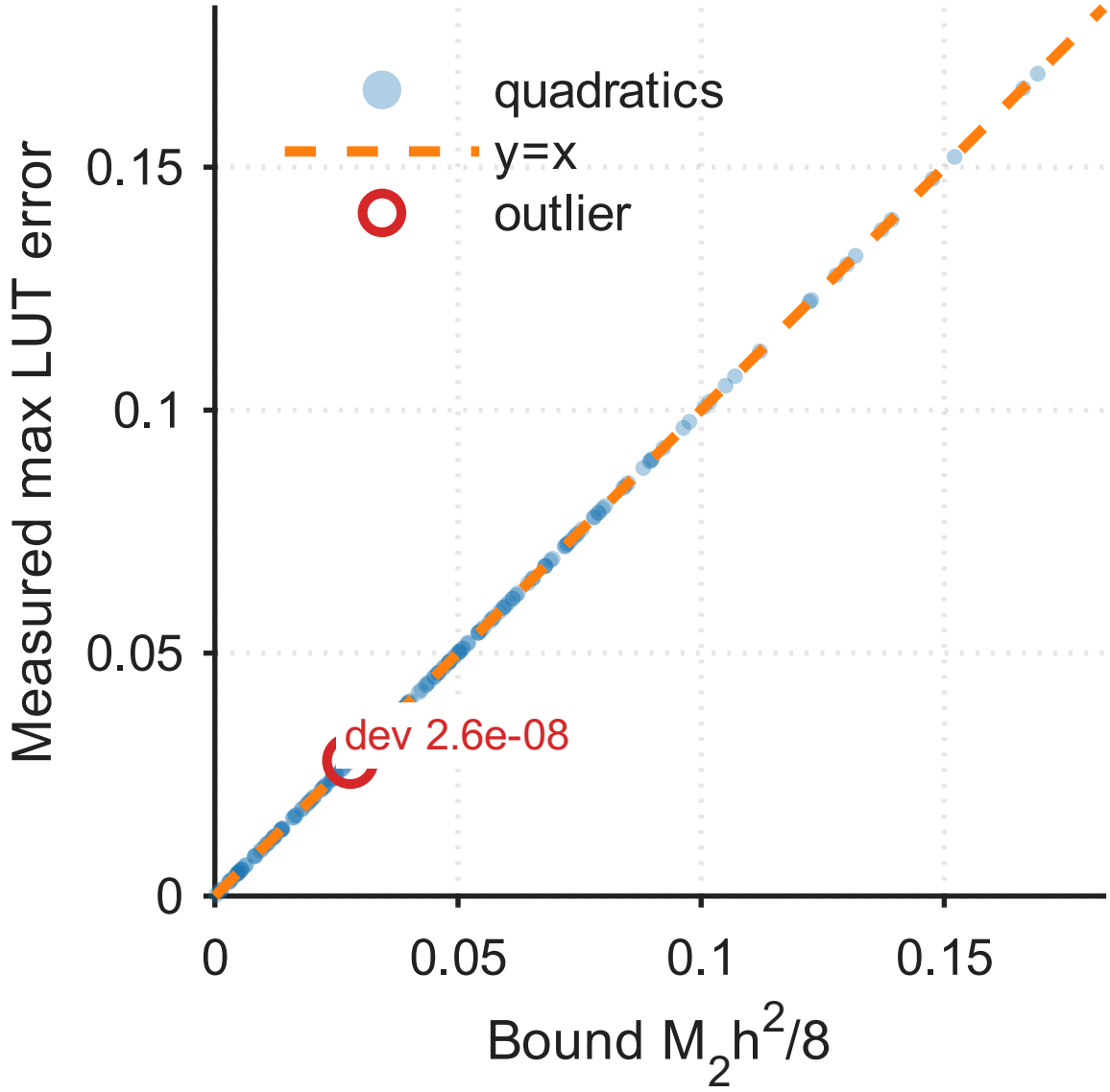
Fig. 4. DA Tightness: Theoretical Bound vs. Actual Maximum LUT Error. 50 representative random C^2 quadratic functions evaluated on N=15 LUT points ( h = 0.429 ). Every point lies exactly on the diagonal y = x , confirming \max_x |f(x) - \text{LUT}(x)| = M_2 \cdot h^2/8 (Theorem C). Extended verification on 1,000 random quadratics: 100% exact match (MATLAB, code/theory/da_tightness_proof.m ). The de Boor bound is not merely an upper bound—it is the best possible uniform bound for the C^2 function class.
