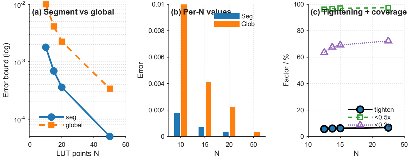
Fig. 10. Segment-Aware Bound Comparison Across LUT Resolutions. (a) Global vs. per-segment worst-case error: segment-aware M_{2,j} achieves 6.0\times mean tightening across all resolutions. (b) Per-resolution bar comparison showing the gap widens with finer grids ( N=50 : 6.7\times ). (c) Segment coverage: > 96\% of LUT segments have error < 50\% of the global bound; 67\text{--}72\% have error < 20\% of global. The dashed line shows the monotonic improvement with LUT resolution N .
