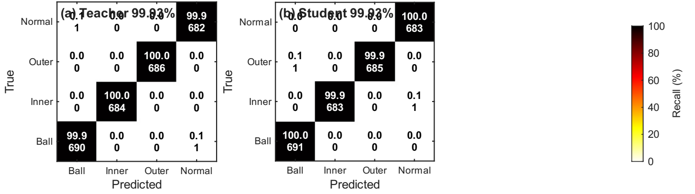
Fig. 13. Confusion matrices. Teacher 1D-CNN (left, 99.93%) and KAN student under VRM-KD (right, 99.93%) on the CWRU held-out test set (2,743 samples). Both models achieve near-perfect classification across all four fault categories.
