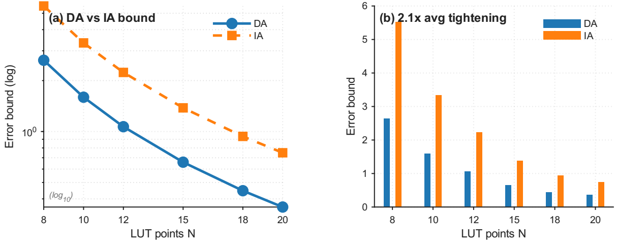
Fig. 9. DA vs. IA Bound Comparison with LUT Resolution. Left: DA achieves 2.1\times tighter bounds than IA across all LUT resolutions ( N = 8\text{--}20 ), decreasing \propto 1/N^2 (Theorem C). At N=15 : DA = 0.66, IA = 1.38 (recomputed from the released checkpoint, 2026-08-03). Right: bar comparison. The gap follows from DA’s Galois-optimality (Theorem B).
