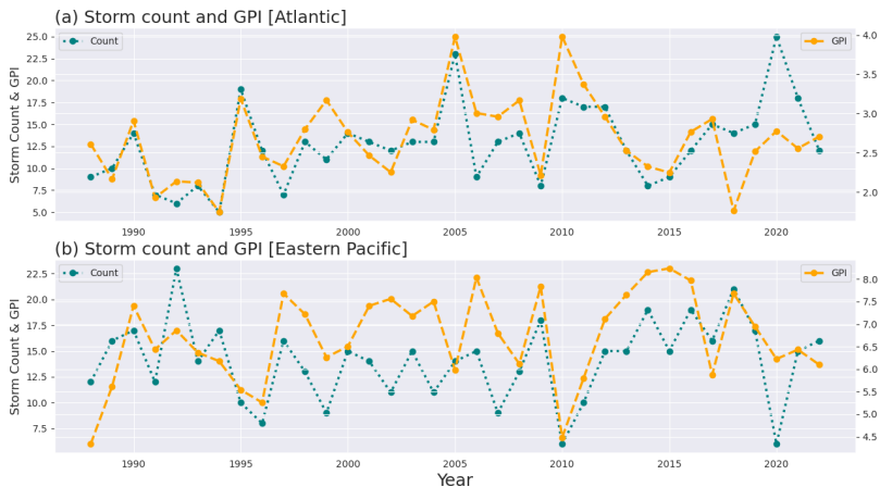
Figure: Tropical cyclone count and area-averaged genesis potential for (a) Atlantic and (b) the eastern Pacific.
