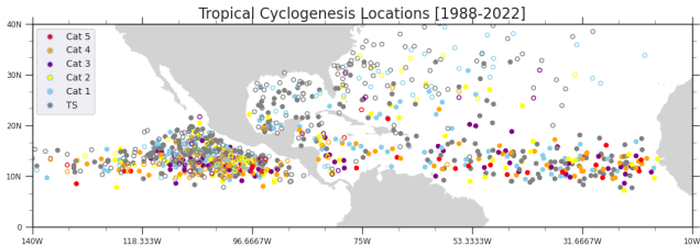
Figure: Genesis Location of Tropical cyclones (1988–2022). Filled circles mark the ones that originated from AEWs. The color of the circles corresponds to the Saffir-Simpson category shown in the figure legend
