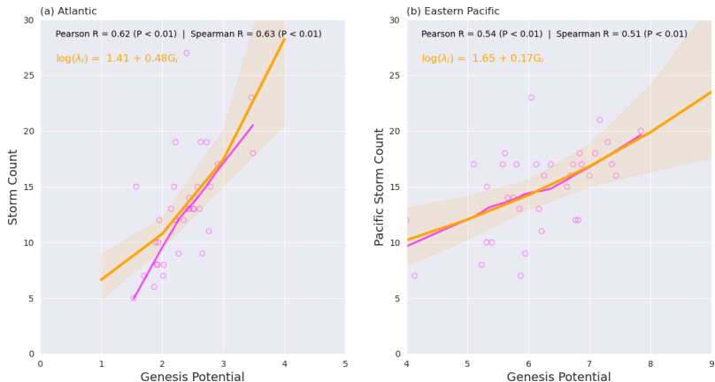
Figure: Relationship between the annual tropical cyclone count and area-averaged genesis potential in the (a) Atlantic and (b) the eastern Pacific. The magenta shows the LOWESS curve while the orange line shows the prediction using Poisson regression. The orange shading denotes the 95% confidence interval for the latter.
