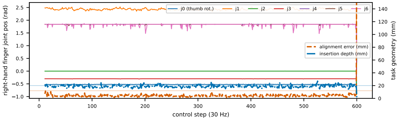
(c) finger joint actions during a successful insertion episode
