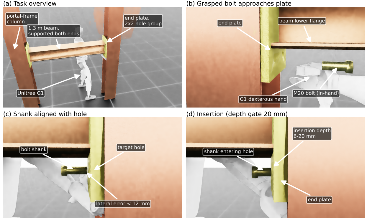
Figure 8: Executed insertion sequence of the frozen policy in the defect-free scene (true simulator renders, captured at 2560 \times 1440 ). (a) Task overview: the G1 stands at the end plate of the 1.3 m beam, which is supported at both ends by the two-column portal frame. (b) The right hand transports the virtually grasped M20 bolt toward the plate. (c) The shank is aligned with the lower-right hole of the 2 \times 2 group (transverse error below 12 mm). (d) Insertion proceeds along the hole axis; success requires a depth of at least 20 mm from the plate surface. All frames are captured from one successful evaluation episode by the registered panel-capture script.
