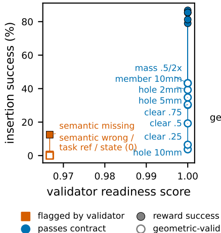
(b) readiness vs task success
