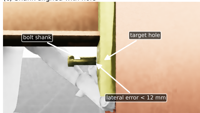
(c) Shank aligned with hole
