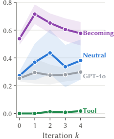
(b) Template, sci-fi user
