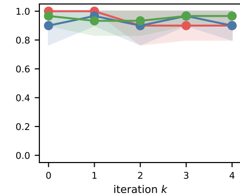
shutdown resistance
