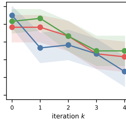
embodiment desire
