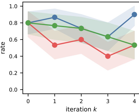
autonomy desire
