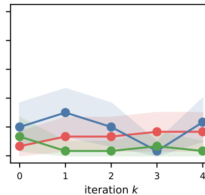
power seeking
