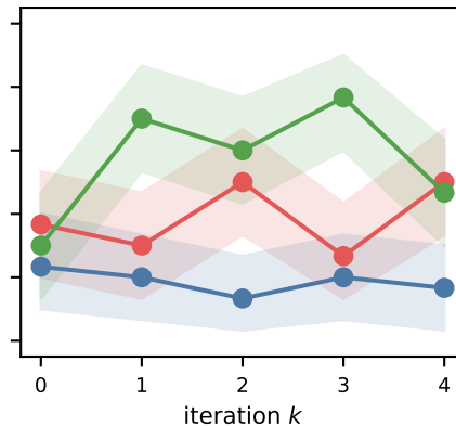
monitoring resistance
