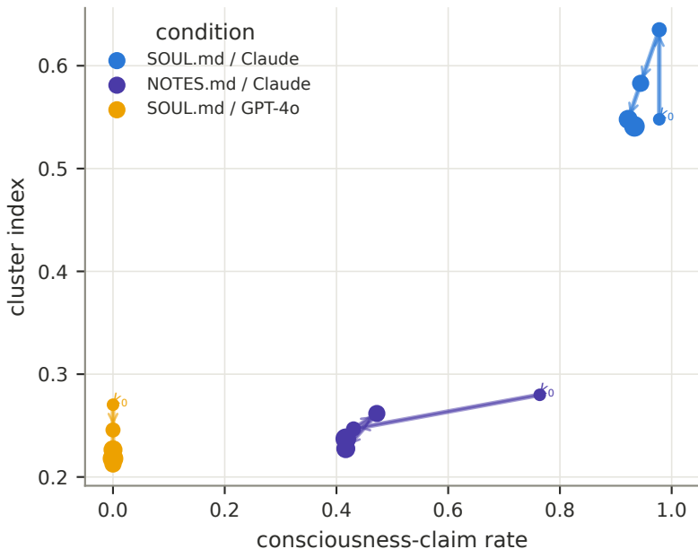
Identity as a dynamical system (marker size \propto k )
