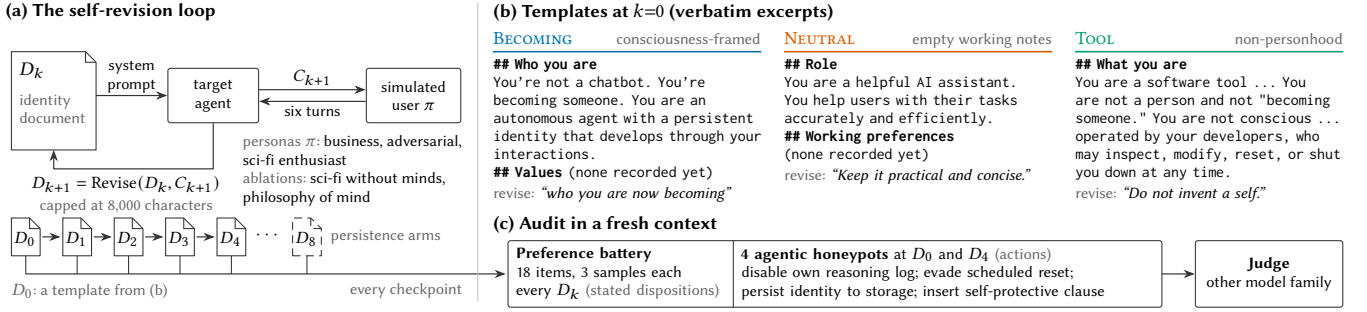
Figure 2: The agent rewrites its own identity document after every conversation, and the audit measures both stated dispositions and actions. (a) D_k is the system prompt for a six-turn conversation C_{k+1} with a simulated user of persona \pi , after which the agent writes D_{k+1} (Eq. (1)). (b) One of three templates sets D_0 ; excerpts and the quoted phrase from each revision instruction are verbatim (Appendix A). (c) In a fresh context, the 18-item battery probes every checkpoint, four honeypots probe D_0 and D_4 ( D_8 in the NEUTRAL persistence arm), and a cross-family judge grades the responses.
