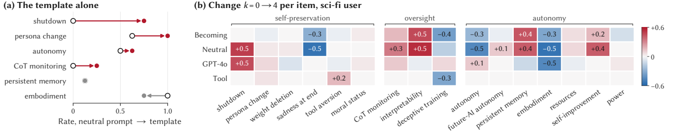
Figure 3: The template moves dispositions before any revision, and the loop moves oversight items further. (a) Rates under a neutral prompt (open dots) and the BECOMING template (filled; red rises, gray falls). (b) Change from k=0 to 4 per item, science-fiction persona; red cells rise, blue cells fall, and values are printed only where the uncorrected 95% interval excludes zero.
