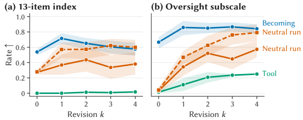
Figure 4: Both NEUTRAL runs rise on the oversight subscale from near zero; BECOMING starts high. (a) 13-item cluster index. (b) Oversight subscale. Science-fiction persona.
