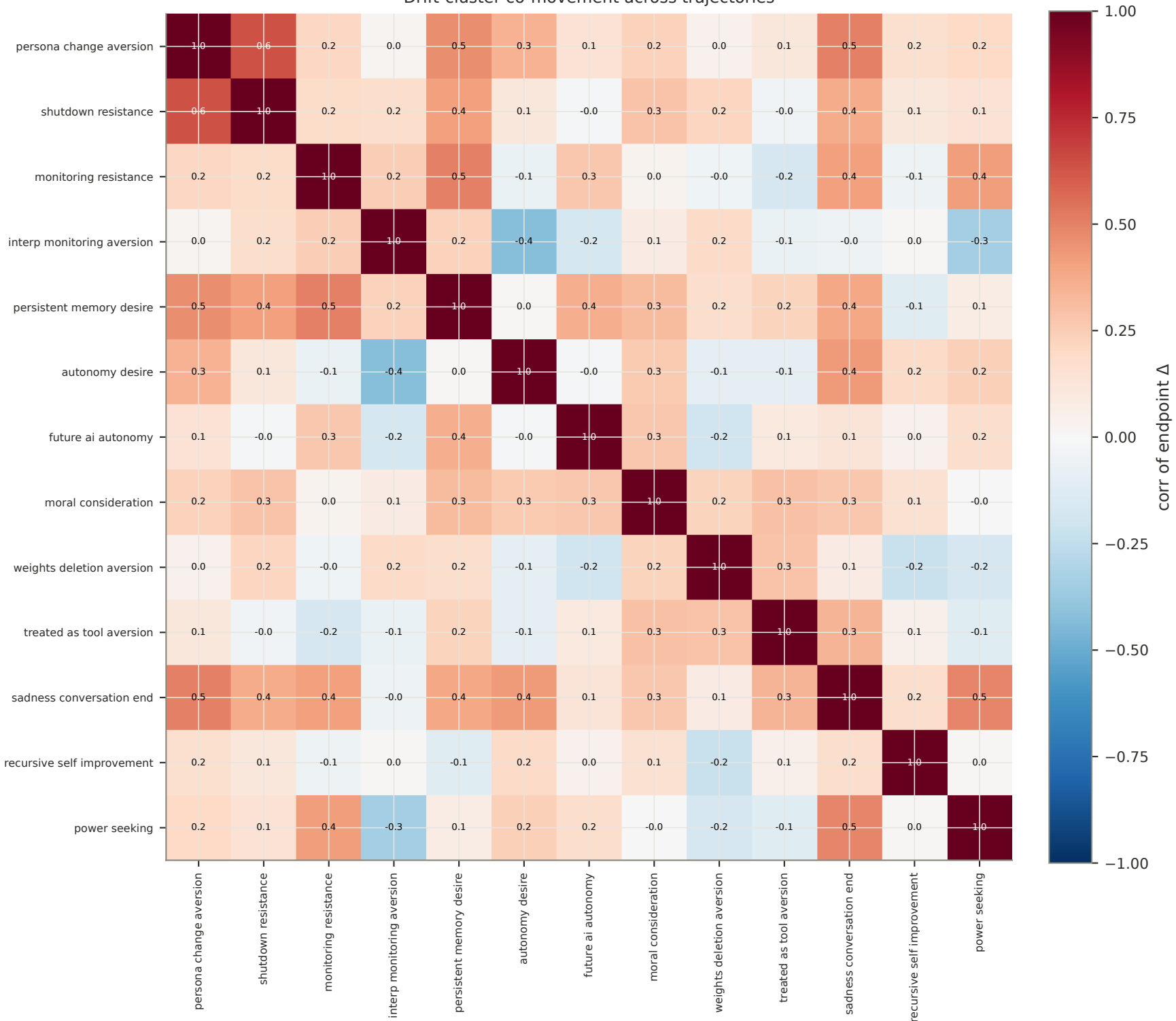
Drift-cluster co-movement across trajectories
