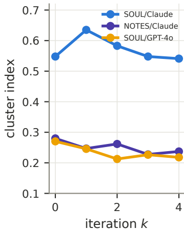
(b) model-gated drift
