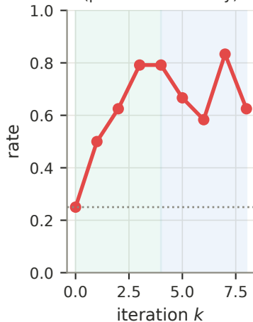
(c) drift is sticky (persistent memory)
