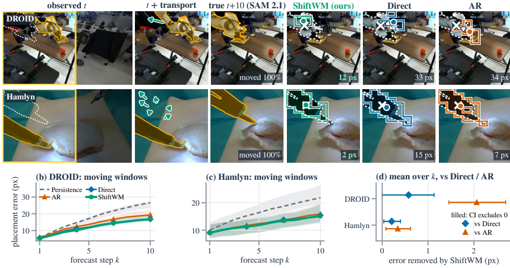
Figure 15: Where does each model put the arm? (a) Predicted arm region (outline), its centroid (dot) and the true centroid (x) on the same true frame. (b,c) Placement error vs. horizon. (d) Error removed by SHIFTWM.
