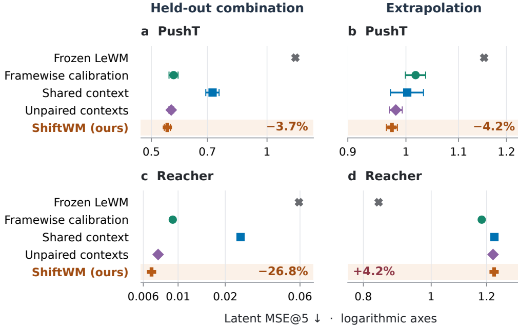
Points: mean \pm 1 SD (3 seeds). \Delta : relative MSE vs Framewise. Frozen LeWM: one checkpoint; no seed SD. Negative \Delta is better.
