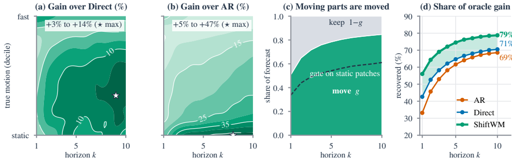
Figure 15: Anatomy of the gains (held-out DROID). (a,b) Error reduction over horizon and motion decile. (c) Gate on moving and static patches. (d) Share of the oracle-gain recovered on moving patches.
