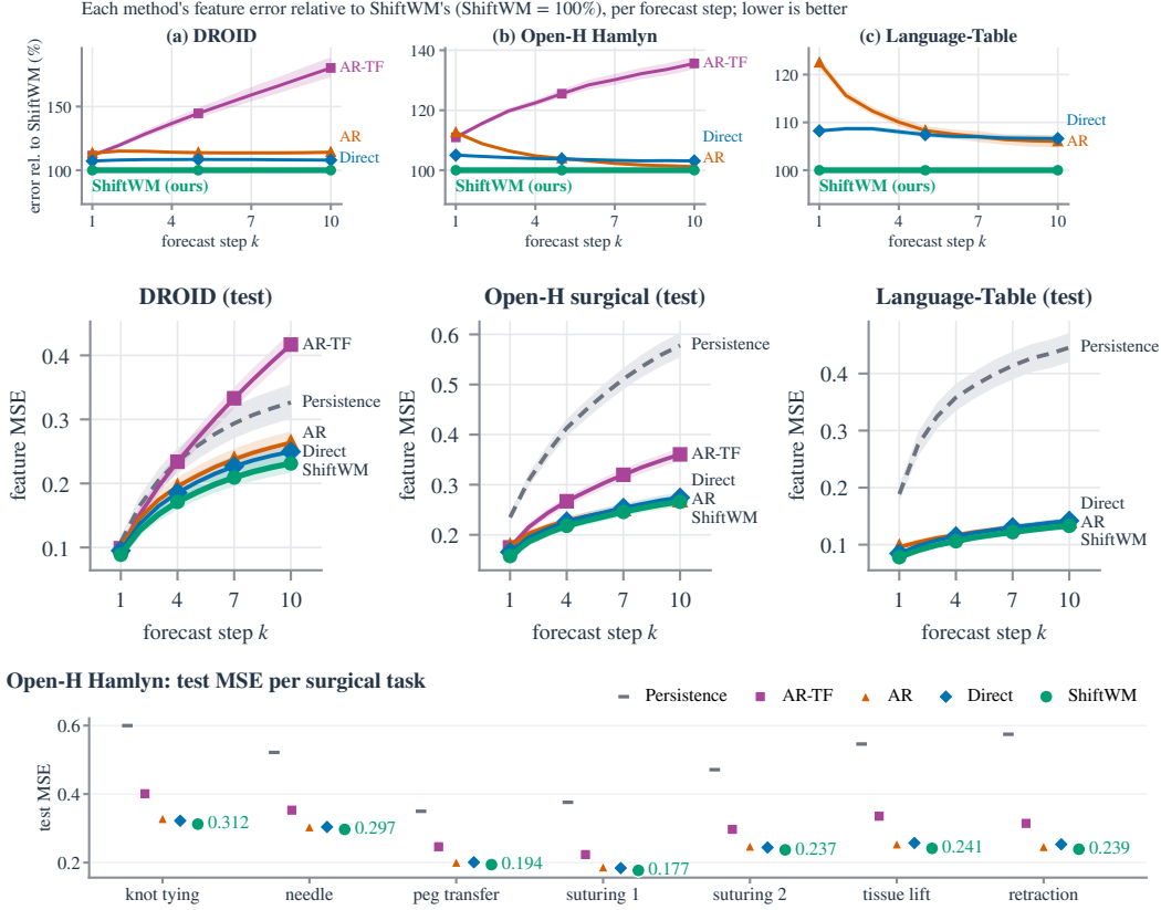
Figure 9: Forecast error per step k and per surgical task. Top: each baseline’s error relative to SHIFTFWM’s (SHIFTFWM = 100%; bands: paired 95% bootstrap). Middle: absolute feature MSE. Bottom: Hamlyn test MSE per task (mean over horizons and 1 seed(s)).
