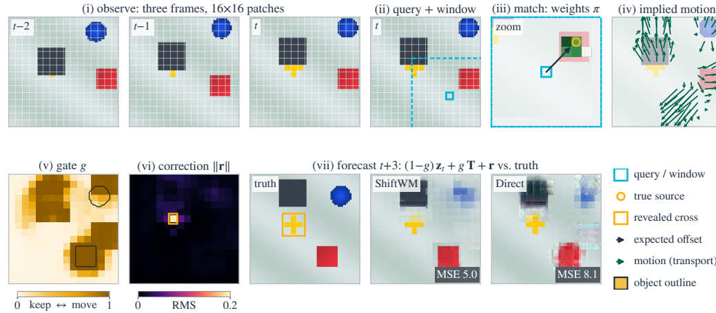
Figure 13: The mechanism on one toy window . (i) Observed frames; (ii) a query patch and its window; (iii) transport weights; (iv) motion where the gate exceeds 0.5; (v) gate; (vi) correction; (vii) forecast at t+3 .
