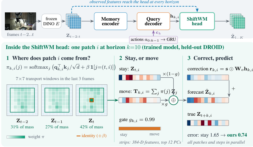
Figure 2: SHIFTMW architecture. For each horizon k , an action-conditioned decoder predicts where every patch comes from (a), whether it moves (b), and a correction (c). Insets are learned outputs on a held-out DROID episode.
