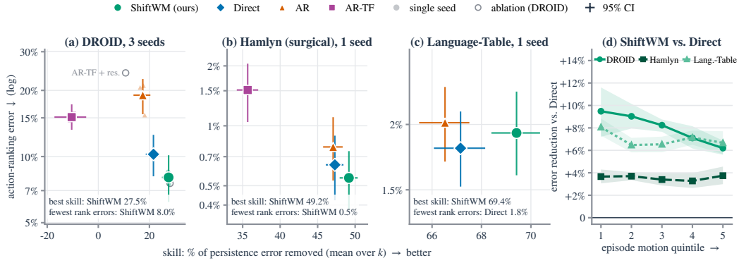
Figure 10: Forecast skill versus action ranking (test) . (a–c) Lower right is better; large markers: seed means with 95% CIs; hollow: DROID ablations. (d) Error reduction of SHIFTWM over Direct per quintile of episode motion.
