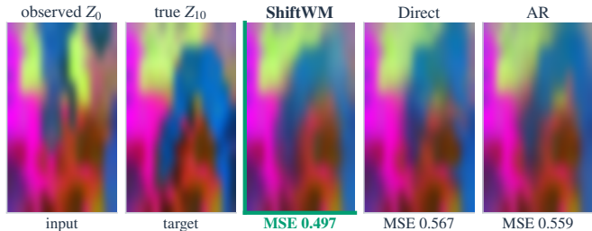
(a) Forecasts in feature space (PCA \rightarrow RGB, k = 10 )
