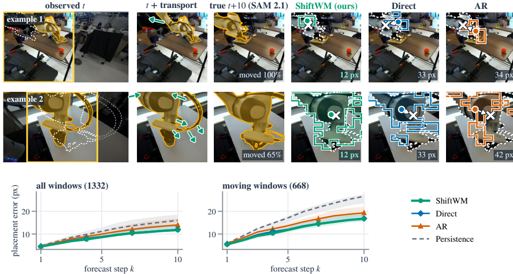
Figure 16: Arm placement, DROID (target: robot arm; 1332 windows, 123 episodes). Same true frame t+10 in every column; examples selected as in Appendix E.2. Bottom: placement error vs. horizon.
