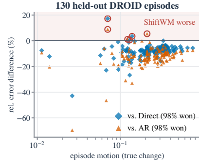
Figure 5: Per-episode gain (DROID test, seed 0, mean over k ; below 0: SHIFTWM better; circles: losses).
