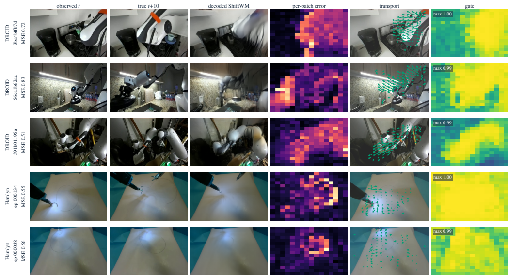
Figure 20: Failure cases.
