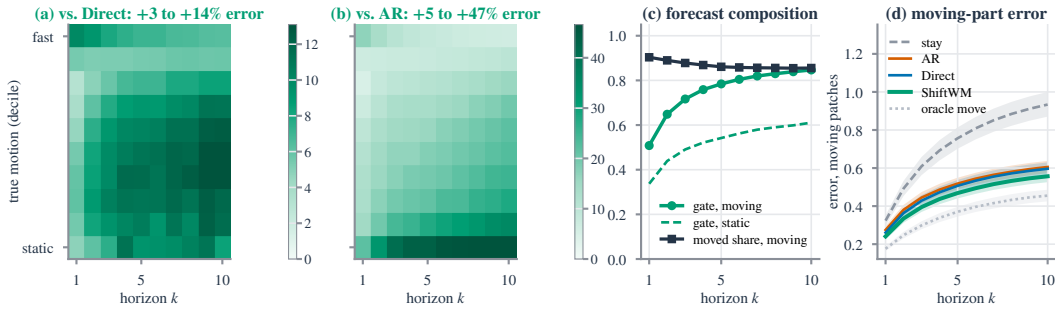
Figure 12: Anatomy of the gains (held-out DROID) . (a,b) Error reduction by horizon and motion decile. (c) Gate and share of the forecast carried by moved features. (d) Moving-part error with 95% CIs.
