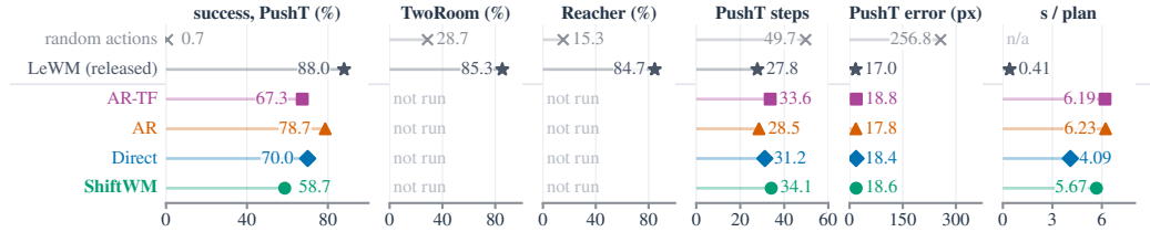
Figure 11: Closed-loop planning , official LeWM protocol (50 episodes \times 3 planner seeds). LeWM and random actions are references; matched predictors are planned on PushT only. Steps: mean to first success (budget 50); error: median final distance to the goal.
