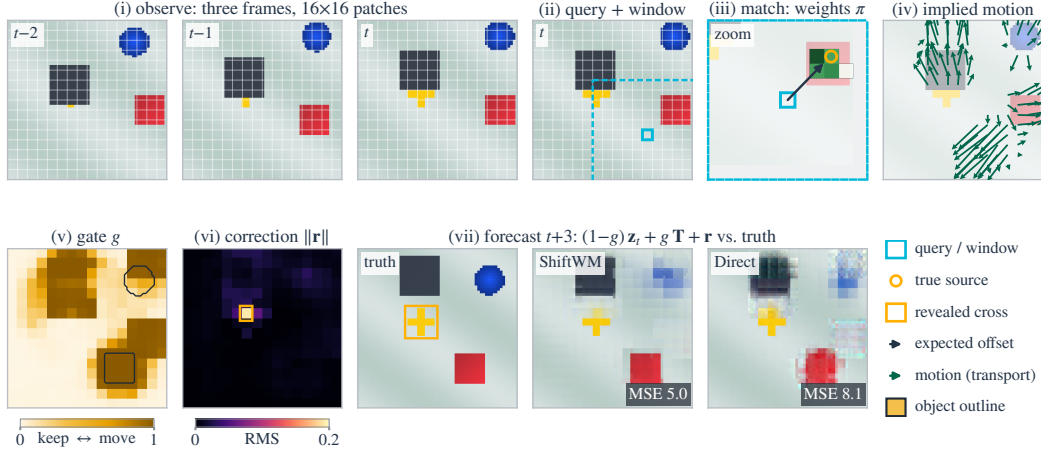
Figure 12: The mechanism on one toy window. (i) Observed frames; (ii) a query patch and its window; (iii) transport weights; (iv) motion where the gate exceeds 0.5; (v) gate; (vi) correction; (vii) forecast at t+3 .
