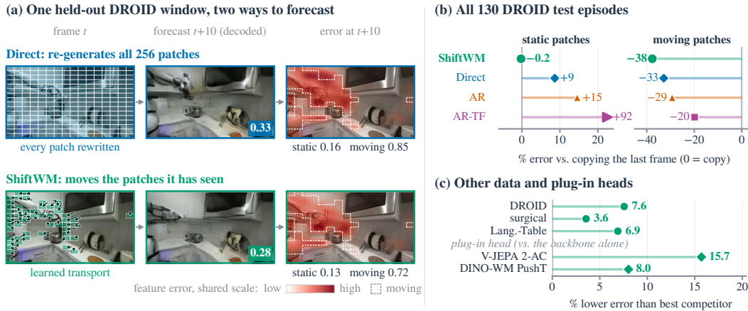
Figure 1: SHIFTWM moves what it has seen instead of regenerating it. (a) One held-out DROID window (Appendix D.8); Direct, a matched regression head, rewrites every patch, whereas SHIFTWM moves the arm’s patches (arrows; dashed: the 25% that change most). (b) Error vs. copying the last frame. (c) % lower error than the best learned competitor.
