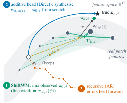
Figure 3: One patch in feature space under the three forecast routes ①–③.
