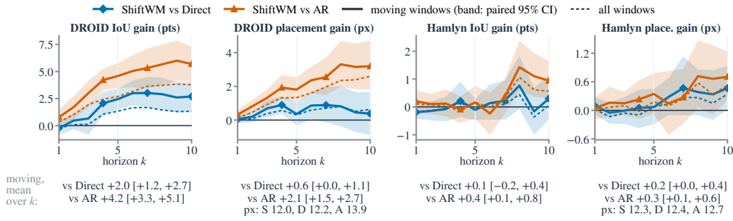
Figure 15: Segmentation read out of the forecasts. Paired gain of SHIFTWM over Direct and AR per horizon: IoU (points) and placement error removed (px of the displayed frame); bands: paired 95% CIs on moving windows. Below: moving-window means over k with CIs, and mean placement error of SHIFTWM (S), Direct (D) and AR (A).
