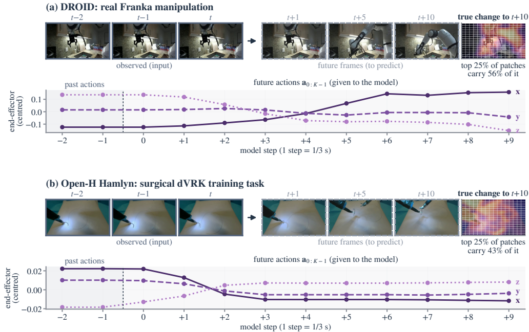
Figure 7: The forecasting task on held-out episodes. Three observed frames and the future actions are given, and the future feature grids are predicted. Right: true feature change over the 16 \times 16 grid.
