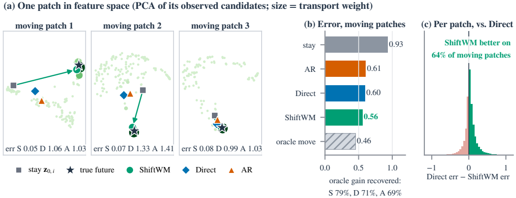
Figure 13: Feature-space geometry on held-out DROID ( k=10 ). (a) Three selected moving patches in a 2-D PCA of their observed candidates. (b) Moving-patch error with the oracle move. (c) Per-patch error difference to Direct.
