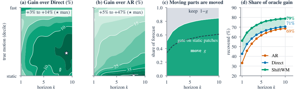
Figure 14: Anatomy of the gains (held-out DROID). (a,b) Error reduction over horizon and motion decile. (c) Gate on moving and static patches. (d) Share of the oracle-move gain recovered on moving patches.
