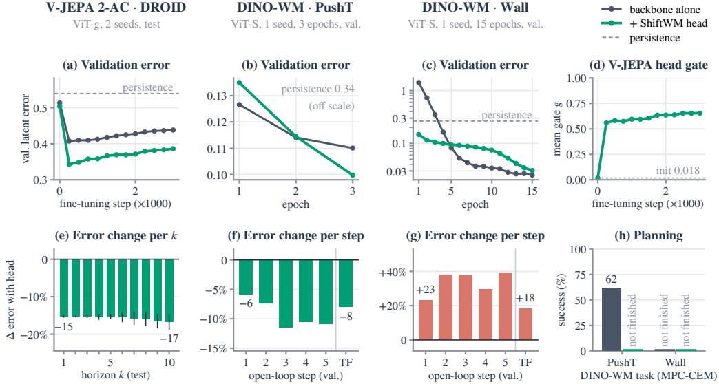
Figure 10: Plug-in heads during training , with (green) and without (dark grey) the SHIFTWM head. (a–c) Validation latent error. (d) Mean V-JEPA gate. (e–g) Change in latent error from the head. (h) DINO-WM planning success.
