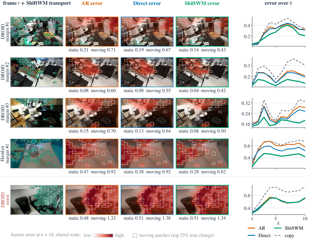
Figure 16: Largest-margin and worst test windows. Top: DROID and Hamlyn windows (top half of motion) with the largest k=10 gain of SHIFTWM over the better of Direct and AR; bottom: SHIFTWM’s worst DROID window. Error maps share one scale (dashed: moving patches). SHIFTWM beats Direct on 98% of DROID test episodes (Figure 5).
