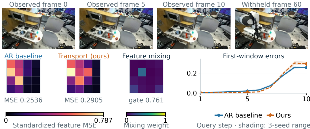
Figure 26: Recorded-video examples and spatial feature errors. Best, median and worst cases use prespecified three-seed episode-level native h10 gain versus the matched 4 × 4 autoregressive baseline. The first eligible window is always shown: the median episode gains +5.358%, but its displayed window regresses by -0.305%. Withheld future frames enter only the evaluator. Images: DROID (CC BY 4.0). Error maps average squared standardized errors over 384 channels and three seeds, with one unclipped scale for all six maps. Curves show mean error and three-seed ranges (not confidence intervals): baseline, solid circles; ours, dashed diamonds. Mixing grids show actual h10 anchor-source weights for target cell (row 2, column 2), averaged across seeds; gates appear below. These are semantic feature mixtures, not physical flow or causal attribution. Population counts and episode- and seed-averaged native-grid endpoint gain appear above. This gain-conditioned validation gallery is not an independent test.
