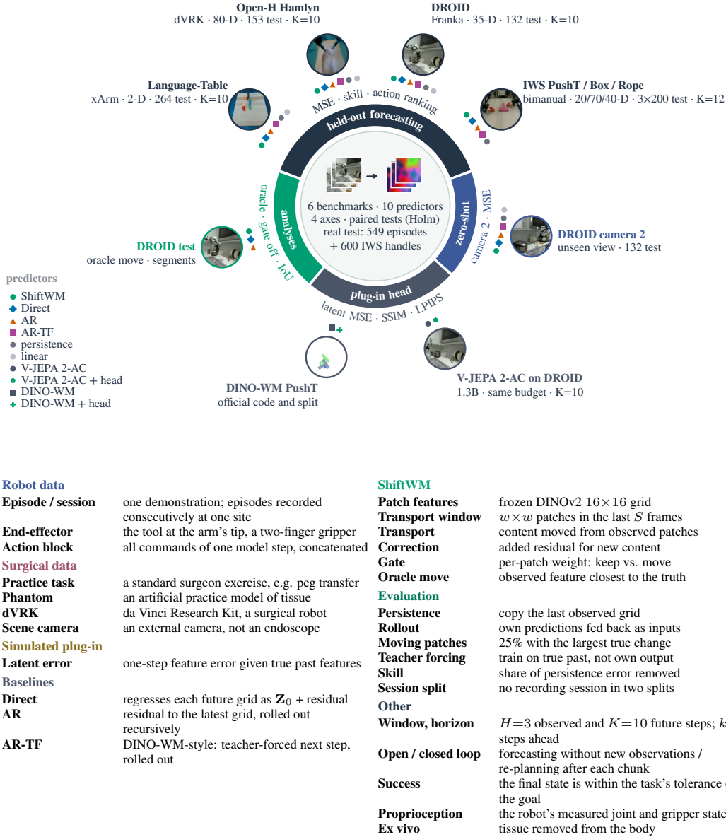
Figure 7: Evaluation overview. Evaluation axes (inner ring, with metrics), benchmarks (real frames) and the predictors evaluated on each (markers). Below: definitions of the other terms.
