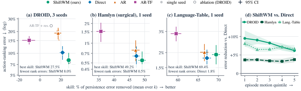
Figure 9: Forecast skill versus action ranking (test). (a–c) Lower right is better; large markers: seed means with 95% CIs; hollow: DROID ablations. (d) Error reduction of SHIFTWm over Direct per quintile of episode motion.
