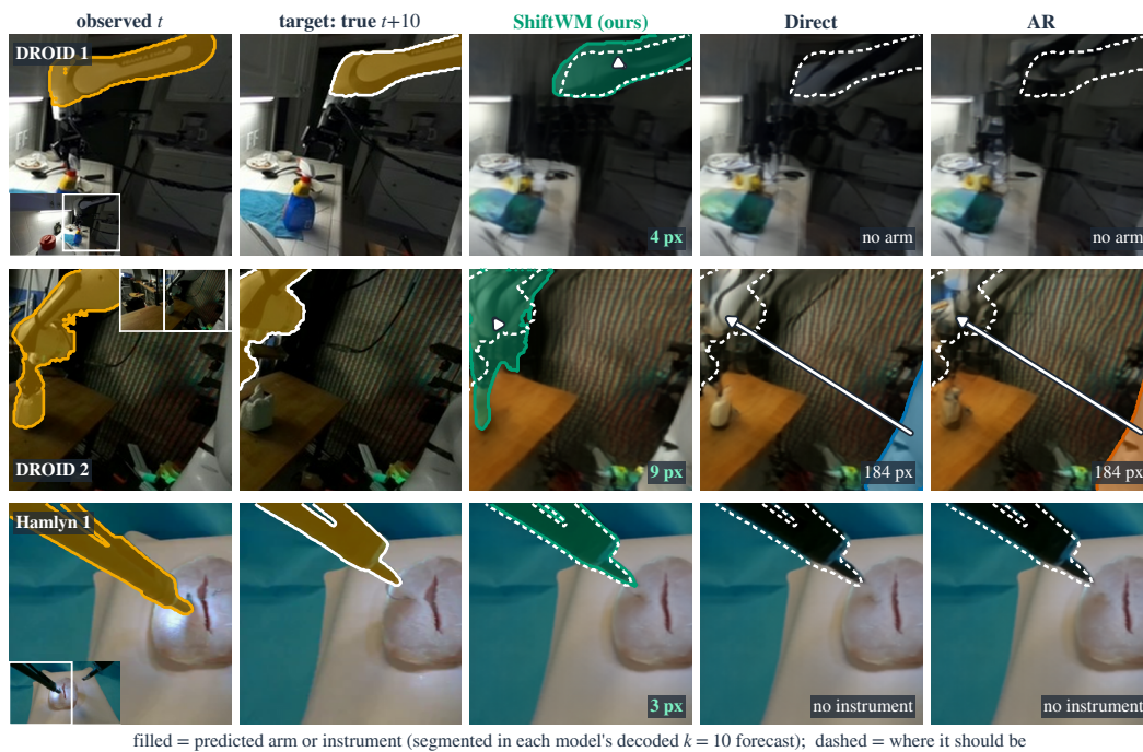
Figure 14: The forecast arm and instruments land where they should. Each column is that method's own decoded k=10 forecast of the same held-out window, segmented with SAM 2.1 (filled; dashed: true position at t+10 ; badges: centroid distance to the true mask).
