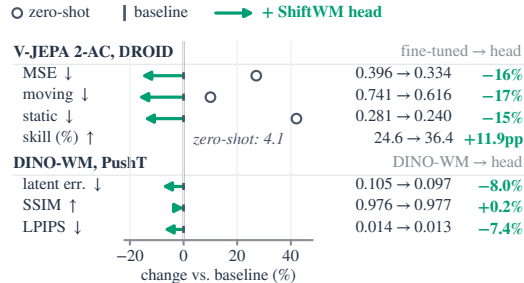
Figure 4: SHIFTWM as a plug-in head : change from adding the head to the same model (same data, schedule, loss). V-JEPA 2-AC: DROID test, base = fine-tuned (2 seeds), circles = zero-shot; DINO-WM: PushT validation. Numbers in Table 3.
