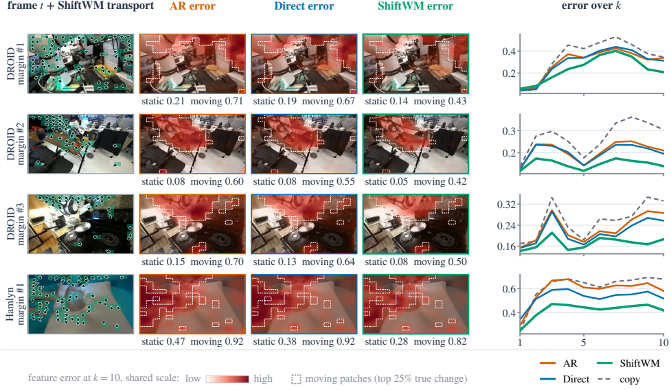
Figure 13: Largest-margin test windows. DROID and Hamlyn windows (top half of motion) with the largest k=10 gain of SHIFTWm over the better of Direct and AR. Error maps share one scale (dashed: moving patches).
