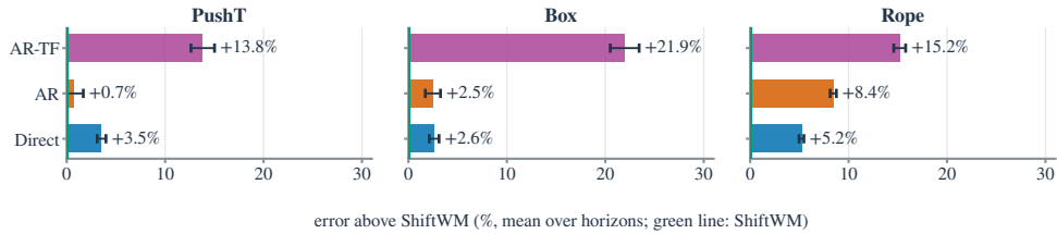
Figure 10: IWS per task . Test error of each matched baseline relative to SHIFTWM on the 200 official validation handles per task (mean over k=1..12 , seed 0; whiskers: paired 95% bootstrap intervals over handles).
