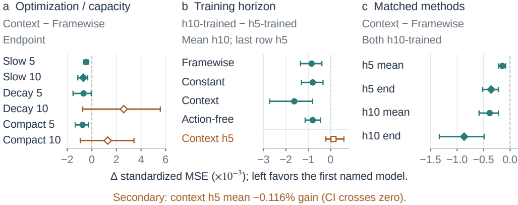
Figure 10: Optimization, capacity and horizon controls for the historical context model (ours), on original DROID validation. Context denotes the factorized two-context model; Constant denotes Constant dynamics. (a) Context minus matched Framewise endpoint MSE under Slow, Decay and Compact interventions, at five or ten action blocks. All 36 runs train 30 epochs and use the common five-query selection objective; Compact changes predictor and context capacity jointly. (b) Ten-query-trained minus original five-query-trained mean MSE on identical ten-query-eligible windows, for every method. The separated final row retains the unfavorable matched-five-query Context secondary result ( -0.116\% relative gain). Training and selection horizons change together. (c) Context minus equally ten-query-trained Framewise on standard populations. Mean averages query errors; end denotes the endpoint. All 12 horizon-study runs train 30 epochs; every selected checkpoint is epoch 1. Bars are paired 95% session/seed bootstrap intervals (10,000 draws); open marks include zero. Axes use different limits but the same MSE unit. Windows are averaged within 141 episodes from 59 sessions and then three seeds equally. Standard h5 uses 1,772 windows; h10 and matched h5 prefixes use 1,631. All four-method absolute errors remain in Tables 21, 26 and 27; all 20 registered horizon contrasts remain in the tables and companion ledger. These exploratory, multiplicity-unadjusted comparisons provide no independent-test claim.
