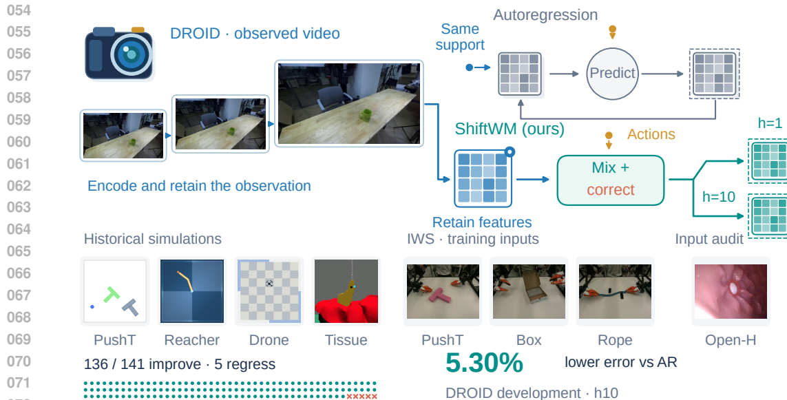
Figure 1: Forecast from retained observations. Three recorded DROID frames supply fixed support features and the last-observed reference Z_0 ; the palette compresses this interface (Figure 2). ShiftWM conditions every query on this support and supplied causal commands; autoregression rolls its own predictions into the next feature history, keeping inferred context fixed. Two schematic endpoints illustrate feature forecasts, not generated RGB; the camera is illustrative. Historical simulations use distinct models; IWS tests a separately trained single-observation adapter; Open-H is a physical-phantom input audit. All 141 DROID development episodes remain visible. The 5.30% reduction compares population mean native, training-standardized h = 10 feature MSE with matched autoregression; uncertainty: Figure 3. Images: DROID/Open-H (CC BY 4.0); IWS (Zhang et al., 2026).
