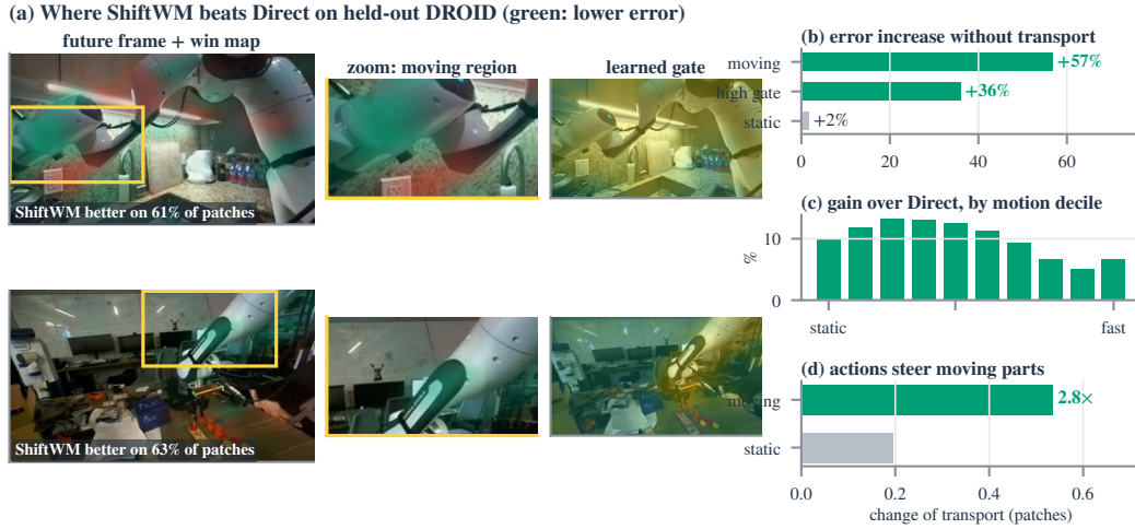
Figure 5: Where and why SHIFTWM wins (held-out DROID, k=10 ). (a) Per-patch error of Direct minus SHIFTWM (green: SHIFTWM lower), with a zoom on the moving region and the learned gate. (b) Removing transport at test time. (c) Gain over Direct per motion decile. (d) Change of the transport field under counterfactual actions.
