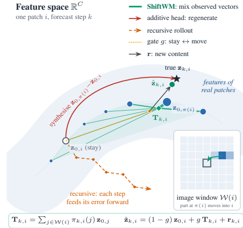
Figure 3: One patch in feature space. SHIFTWM mixes observed vectors (Prop. 1); additive heads regenerate the displacement (Prop. 2); recursion drifts (Prop. 3).
