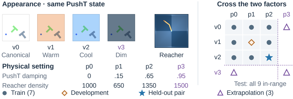
Figure 12: Crossed appearance and dynamics in the historical simulation study. Full recorded simulator frames illustrate PushT and Reacher. The four PushT views apply the exact RGB transforms to one state; physical settings change damping or arm and finger density together. Training and ordinary validation use seven pairs; (v_1, p_1) is development and (v_2, p_2) is held-out composition. Three additional pairs use new factor values; blank cells are unevaluated. Independent test trajectories cover all nine in-range pairs, including familiar combinations. Trajectory seeds are split before paired rendering; factor IDs are unavailable to the deployed model. This is the historical context-model protocol.
