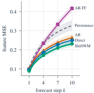
DROID (test)
