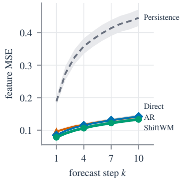
Language-Table (test)
