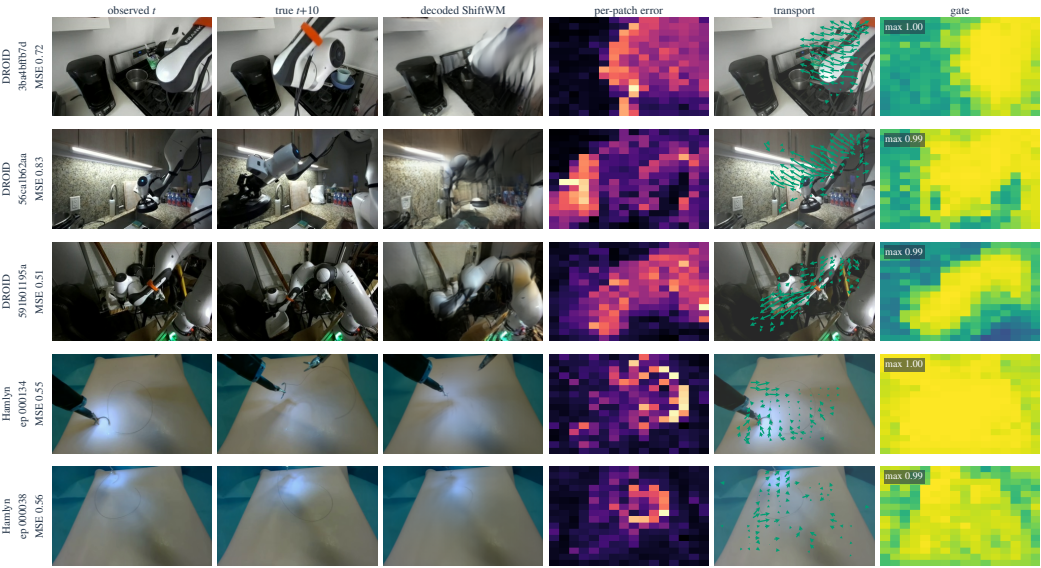
Figure 21: Failure cases.
