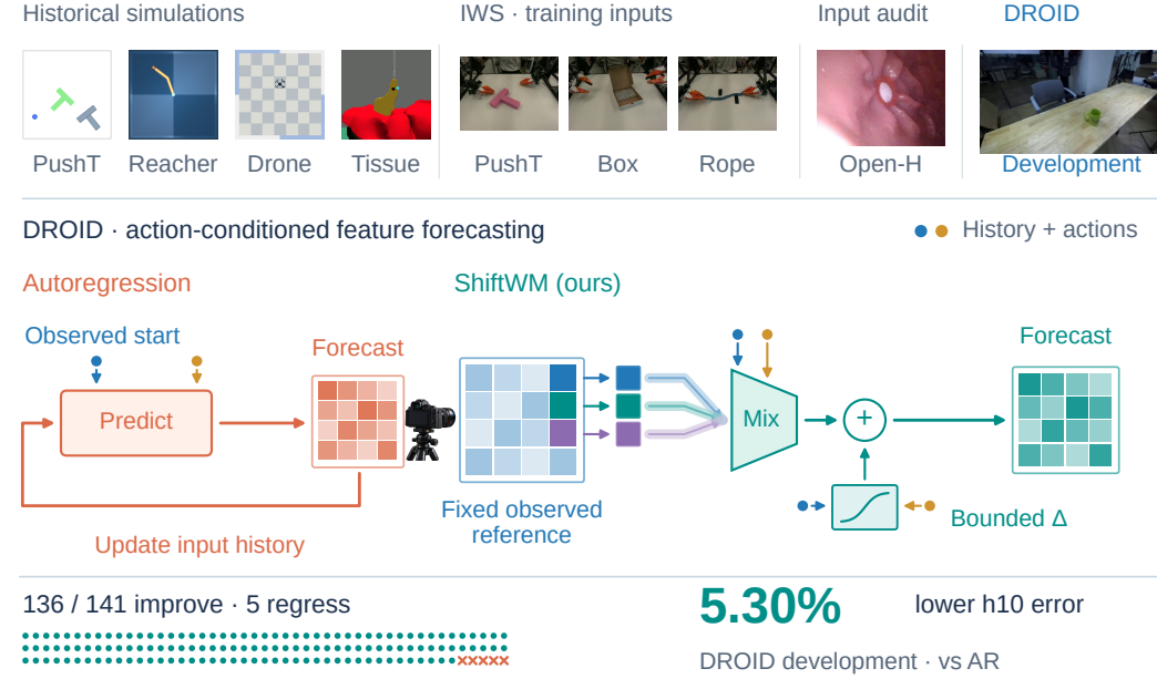
Figure 1: Retain observations while forecasting. Autoregression feeds its own prediction into the next three-frame input history; ShiftWM retains the observed reference. Mix includes the gate in W = (I - D) + DT ; a projected tanh correction has unit coordinate bound after training standardization. For ShiftWM, blue/gold ports abbreviate conditioning through H_h on fixed observed support and causal action prefixes (Figure 2). Three colored source locations illustrate mixing, not measured weights; grids are schematic features, not generated RGB, and the camera is illustrative. Gallery: historical simulations use distinct context models; IWS inputs belong to ongoing training; Open-H is a physical-phantom input audit only. Bottom: all 141 DROID development episodes. The 5.30% reduction compares population mean native, training-standardized h10 feature MSE with matched autoregression; uncertainty appears in Figure 3. Images: DROID and Open-H (CC BY 4.0); IWS (Zhang et al., 2026). Simulator attribution and selection rules accompany the editable figure.
