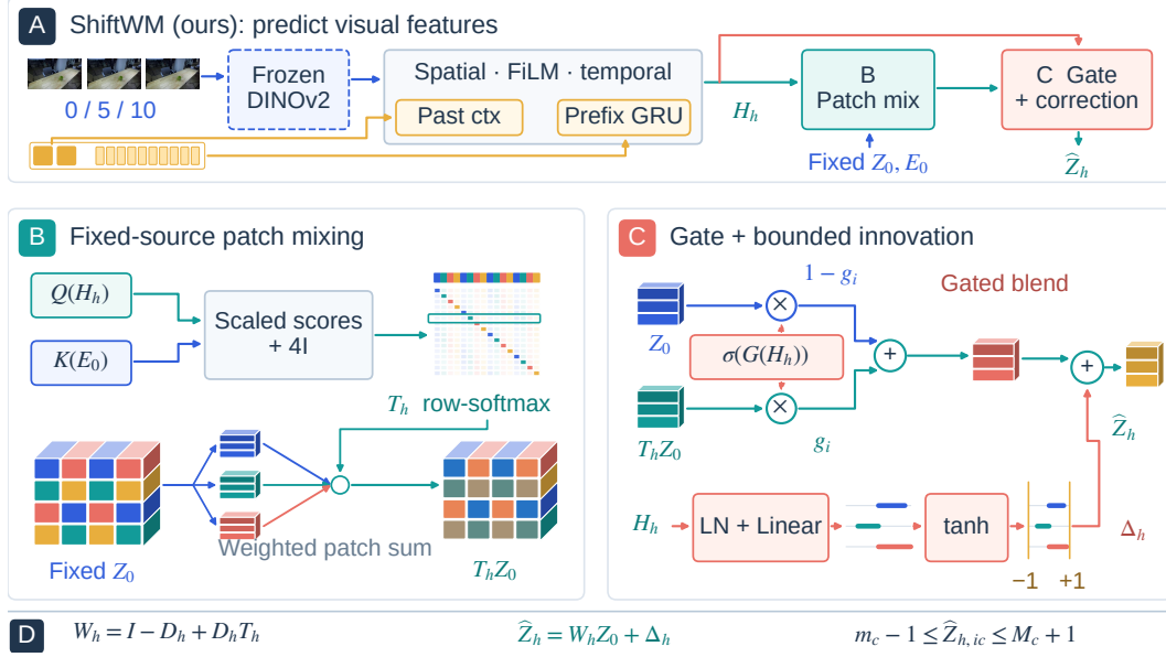
Figure 2: ShiftWM (ours), with expanded decoder operations. (A) The DROID instantiation receives recorded frames 0/5/10 and supplied action blocks. Frozen DINOv2 features are pooled to 4 \times 4 and standardized using fixed training-only channel statistics. The compact causal module contains spatial encoding, past-only patch-mean context, FiLM, a chronological action GRU and the temporal predictor; only the command prefix through h is used. (B) Keys use fixed E_0 \in \mathbb{R}^{16 \times 96} , the last spatial encoding before FiLM; queries use the horizon state H_h . T_h = \text{softmax}_{\text{row}}(Q(H_h)K(E_0)^\top / \sqrt{96} + 4I) mixes the fixed normalized observation Z_0 \in \mathbb{R}^{16 \times 384} . (C) The per-patch affine sigmoid gate combines direct and mixed sources. An independent branch applies LayerNorm and an affine 96 \rightarrow 384 projection to the same H_h , then \Delta_h = \tanh(R(H_h)) is added after blending. (D) D_h = \text{diag}(g_h) , W_h \geq 0 , W_h \mathbf{1} = \mathbf{1} , and \hat{Z}_h = W_h Z_0 + \Delta_h ; m_c, M_c are the observed channel minimum and maximum. The envelope concerns standardized coordinates, not prediction error. Panels B/C expand the named modules; dashed arrows denote gate coefficients. Feature objects, mixing weights and activation bars are schematic, not generated RGB. Unchanged DROID photographs are CC BY 4.0. Only DINOv2 weights are frozen; predictor modules train offline.
