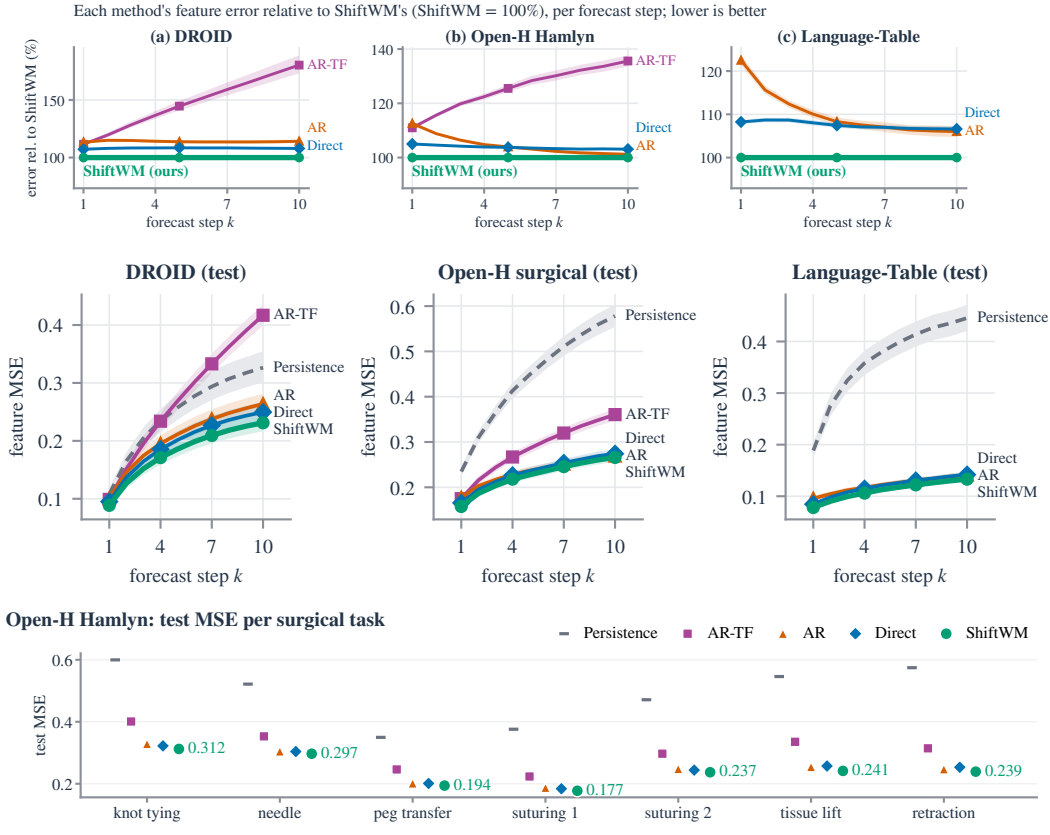
Figure 8: Forecast error per step k and per surgical task. Top: each baseline's error relative to SHIFTWM's (SHIFTWM = 100%; bands: paired 95% bootstrap). Middle: absolute feature MSE. Bottom: Hamlyn test MSE per task (mean over horizons and 1 seed(s)).
