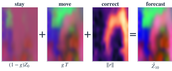
(b) How ShiftWM composes a forecast
