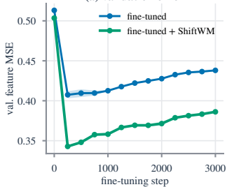
(a) validation error
