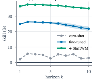
(c) test skill per horizon
