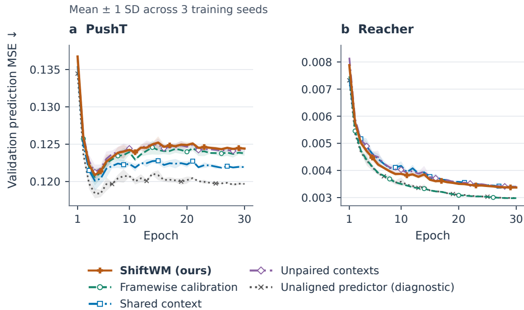
Figure 13: Validation prediction loss over the completed training campaign. Curves and shaded bands show means and sample standard deviations over three training seeds at common logged epochs. Colors and line styles identify model variants. No future epochs are extrapolated, and bands are not confidence intervals. The two panels have separate vertical scales. These are validation records, not test-set or planning-performance results.
