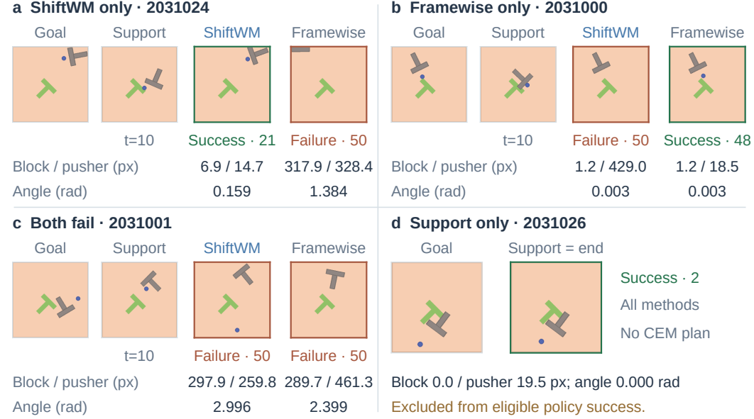
Figure 16: Matched PushT outcomes, including success before planning. Recorded simulator observations compare the historical ShiftWM (ours) context model with Framewise, at training seed 0 on development ( v_1, p_1 ). These are the original first-lexicographic cases from four outcome strata, not success-frequency estimates. Each card shares pixel-identical goal and support observations across methods. Success/failure labels give the actual native stopping call; endpoints are not synchronized. The scored goal is the gray block and blue pusher in the goal image. The persistent green T is an unscored reset marker. Block and pusher errors use native 512 \times 512 coordinates despite the 224 \times 224 recorded images. Success requires their combined position-error norm below 20 pixels and wrapped block-angle error below \pi/9 . In (b), 1.2 pixels of block error does not compensate for 429.0 pixels of pusher error. In (d), every method reaches the goal during shared support at call 2; the support and terminal image is identical and shown once. No CEM plan executes. This raw success is excluded from eligible policy success and is not evidence of planner competence; no eligible joint-success PushT case exists in this population. The allowance is 50 native calls including support. All Shared-context outcomes and intermediate observations remain in the complete archived gallery; no displayed image is an RGB prediction.
