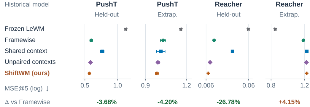
Figure 12: Historical context model: complete forecast comparison. Each panel retains all five aligned methods. Points and bars show means and sample SD across three training seeds; Frozen LeWM has one checkpoint and no seed SD. The target is fixed-reference latent MSE after five recursive blocks (25 native actions), using recorded future actions. Axes are logarithmic with panel-specific limits; latent coordinates differ between environments. The last row is the signed relative MSE change of ShiftWM (ours) versus Framewise: negative is better, with no interval or significance inference. Reacher extrapolation is unfavorable, and Frozen LeWM has its lowest mean. The unaligned diagnostic remains in the complete table, outside this aligned comparison. These are forecasting results for the earlier model, not closed-loop success or evaluation of the newer spatial architecture.
