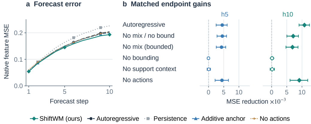
Figure 3: Forecast profiles and matched component gains on DROID development. (a) All 50 mean native feature errors for the five original methods; one forecast step spans five native commands. (b) All six controls at h5/h10: comparator-minus-ShiftWM MSE with paired 95% recording-session \times seed bootstrap intervals (10,000 draws, seed 173). Right of zero favors ShiftWM (ours); open marks include zero. “No mix/no bound” is the additive anchor; “No mix (bounded)” adds bounding. Omitting bounding is slightly better at h5, with both native intervals including zero. The six component follow-up models were added after the original controls were revealed. Table 1 retains all endpoint scores; Tables 10 and 11 retain all 36 contrasts, including coarse-coordinate regressions and interactions.
