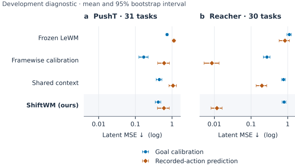
Figure 18: Prediction and goal calibration are distinct errors. Posthoc development diagnostics for frozen LeWM and three seed-0 trained models. Both errors are per-dimension MSE in fixed pre-trained coordinates against the same canonical goal; lower is better. Blue circles denote goal calibration; orange diamonds use the five recorded future action blocks. Horizontal axes are logarithmic so small errors remain visible. Error bars are 95% trajectory-seed bootstrap intervals, excluding common support-only successes; they do not measure training-seed variation. Small recorded-action prediction error alone does not establish accurate goal calibration or successful planning.
