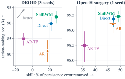
Figure 4: Better forecasts without weaker action sensitivity. Skill vs. action-ranking accuracy (95% CIs); SHIFTWM is highest on both axes on DROID and Open-H.
