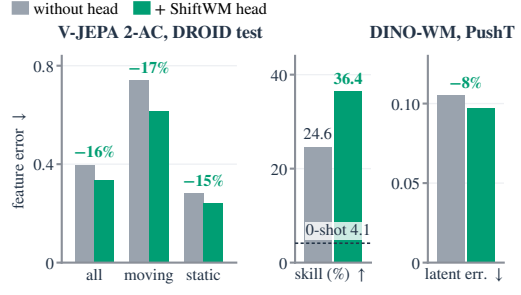
Figure 5: SHIFTWM as a plug-in head. Same model, data, schedule and loss with and without the head. V-JEPA 2-AC: DROID test, 2 seeds (dashed: released model, zero-shot); DINO-WM: PushT validation.
