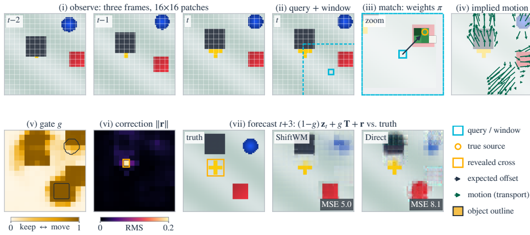
Figure 13: The mechanism on one toy window. (i) Observed frames; (ii) a query patch and its window; (iii) transport weights; (iv) motion where the gate exceeds 0.5; (v) gate; (vi) correction; (vii) forecast at t+3 .
