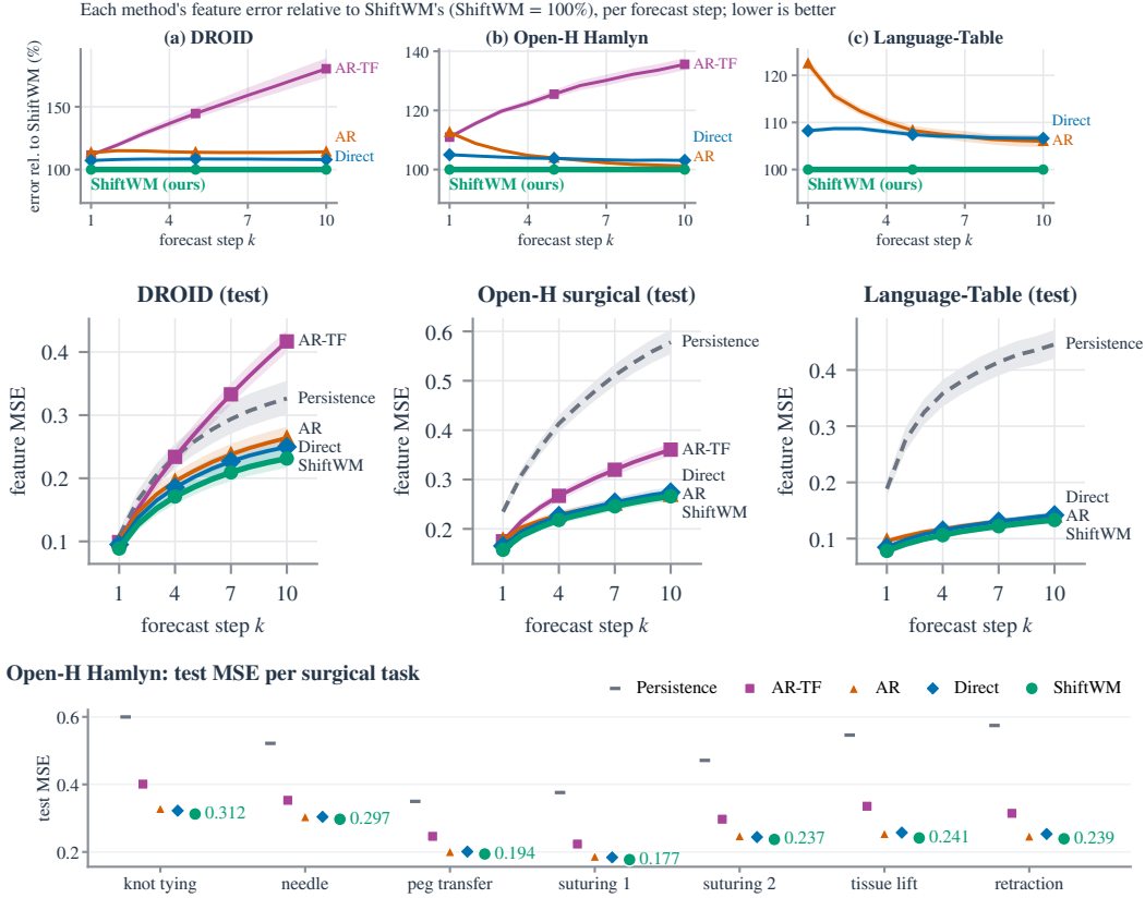
Figure 9: Forecast error per step k and per surgical task. Top: each baseline’s error relative to SHIFTWm’s (SHIFTWm = 100%; bands: paired 95% bootstrap). Middle: absolute feature MSE. Bottom: Hamlyn test MSE per task (mean over horizons and 1 seed(s)).
