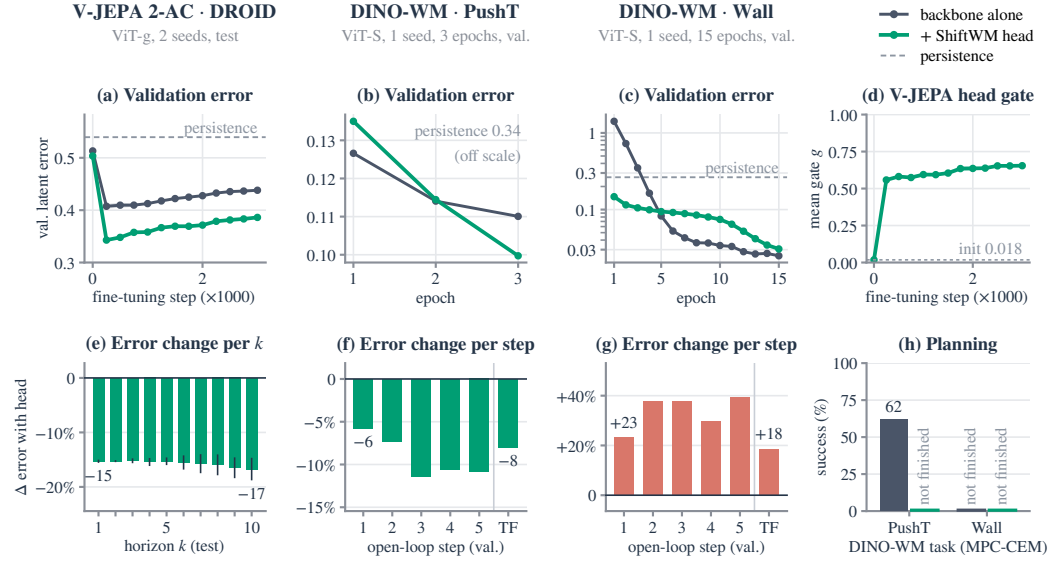
Figure 11: Plug-in heads during training , with (green) and without (dark grey) the SHIFTWm head. (a–c) Validation latent error. (d) Mean V-JEPA gate. (e–g) Change in latent error from the head. (h) DINO-WM planning success.
