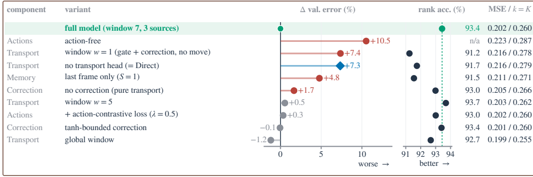
Figure 6: Ablations on DROID validation (seed 0; selection on validation only), sorted by \Delta , the change of validation MSE against the full model (positive = worse); action-ranking accuracy and absolute MSE on the rigt.
