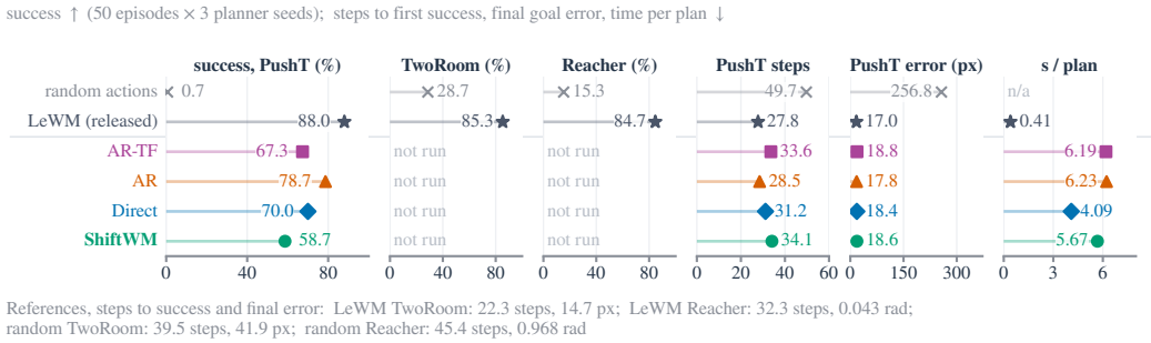
Figure 12: Closed-loop planning , official LeWM protocol (50 episodes \times 3 planner seeds). LeWM and random actions are references; matched predictors are planned on PushT only. Steps: mean to first success (budget 50); error: median final distance to the goal.
