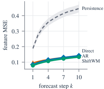
Language-Table (test)
