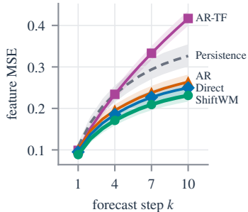
DROID (test)
